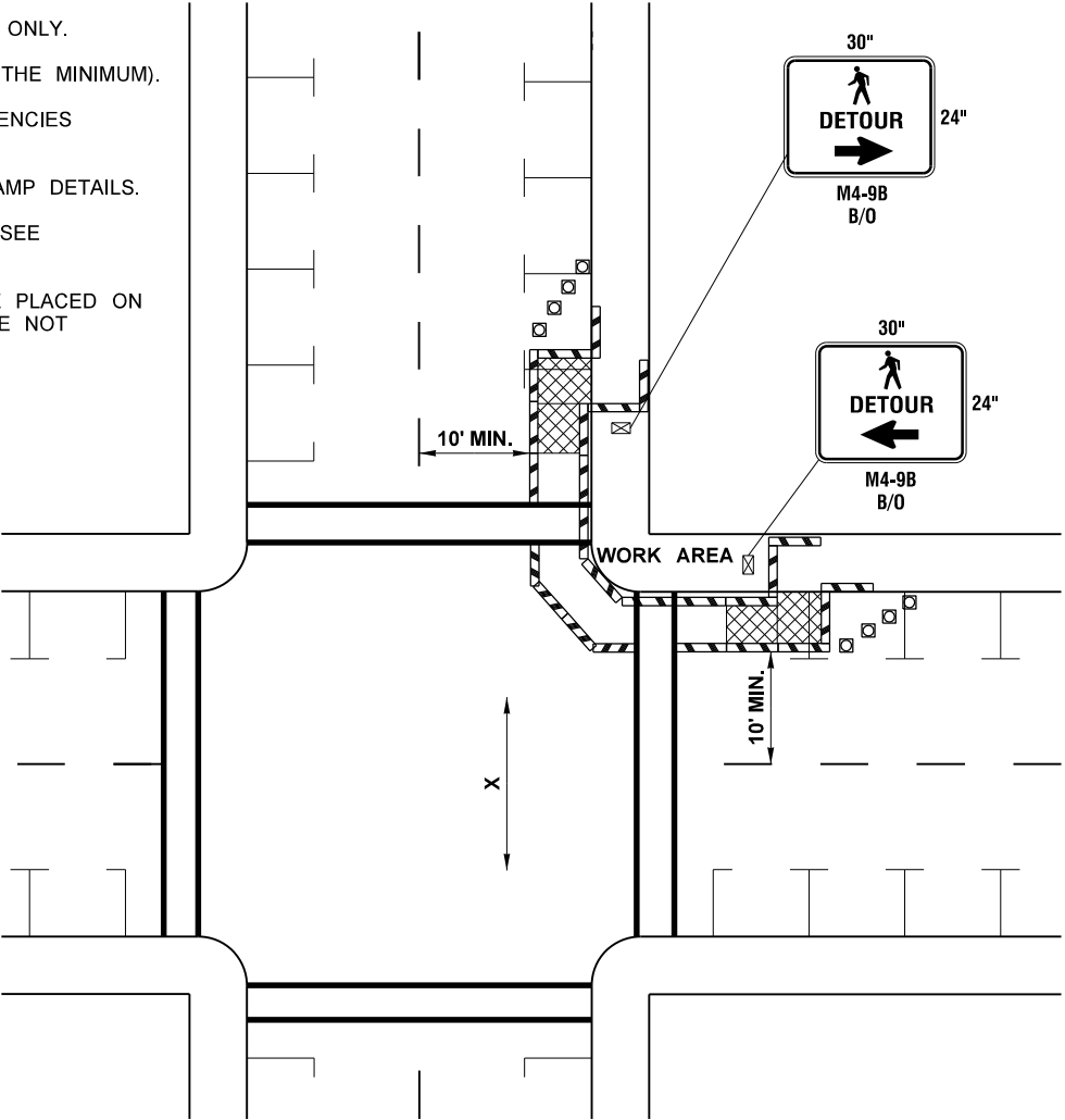
SIDEWALK DIVERSION
