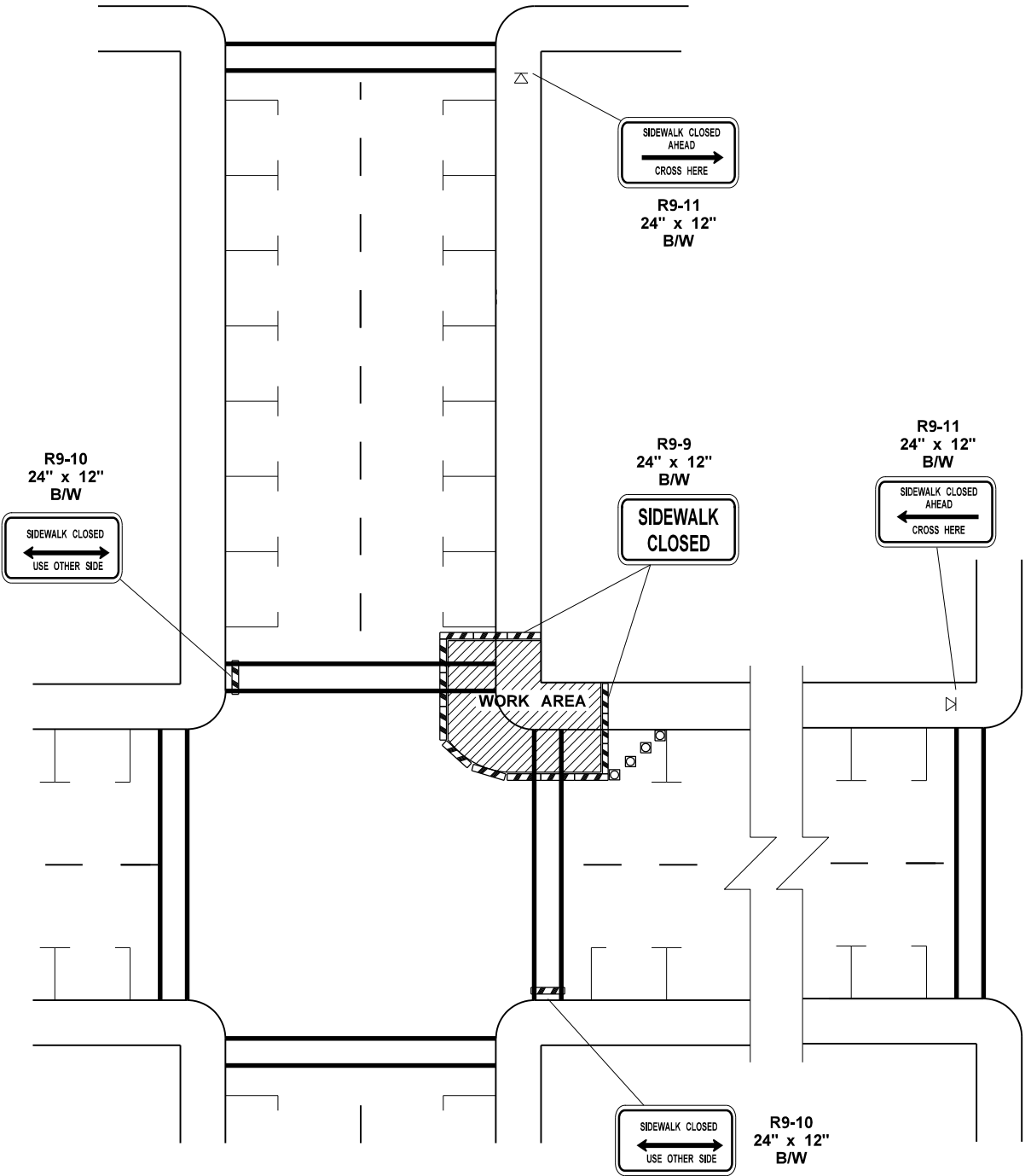
SIDEWALK DETOUR
